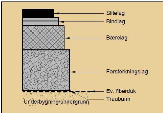
Figur 6.5: Overbygning
