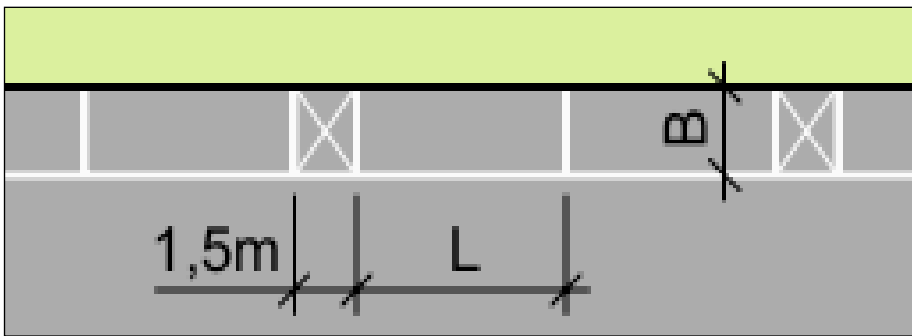
Figur 4.42: Parkering langs kantstein
